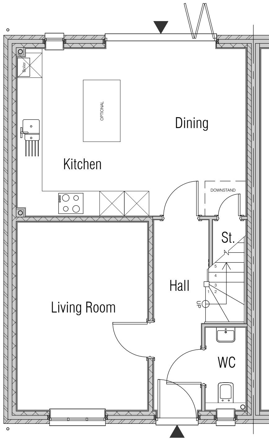
Plot 17 Ground floor
