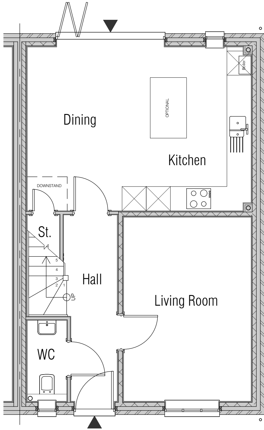
Plot 14 Ground floor
