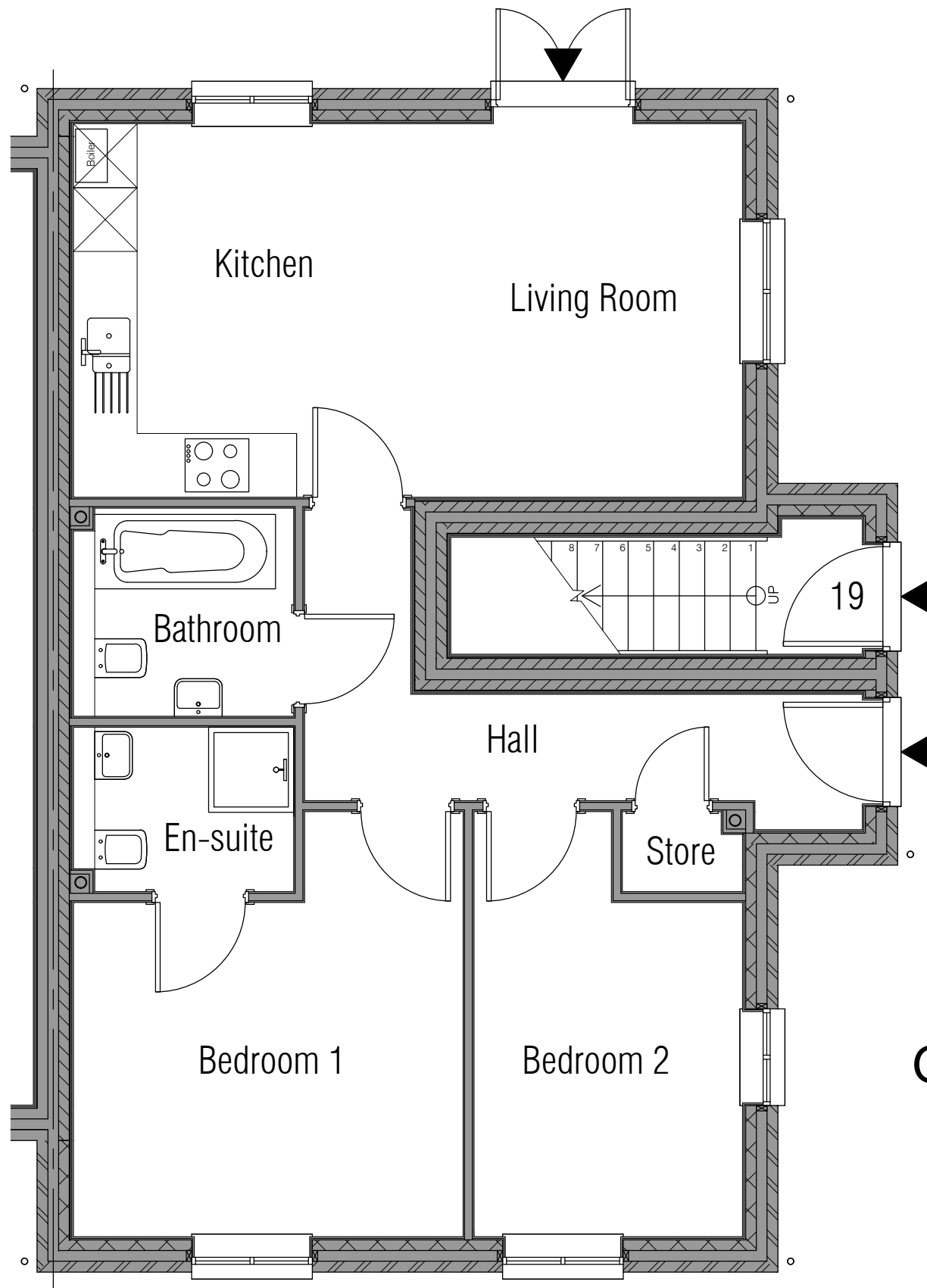
Plot 18 Ground floor
