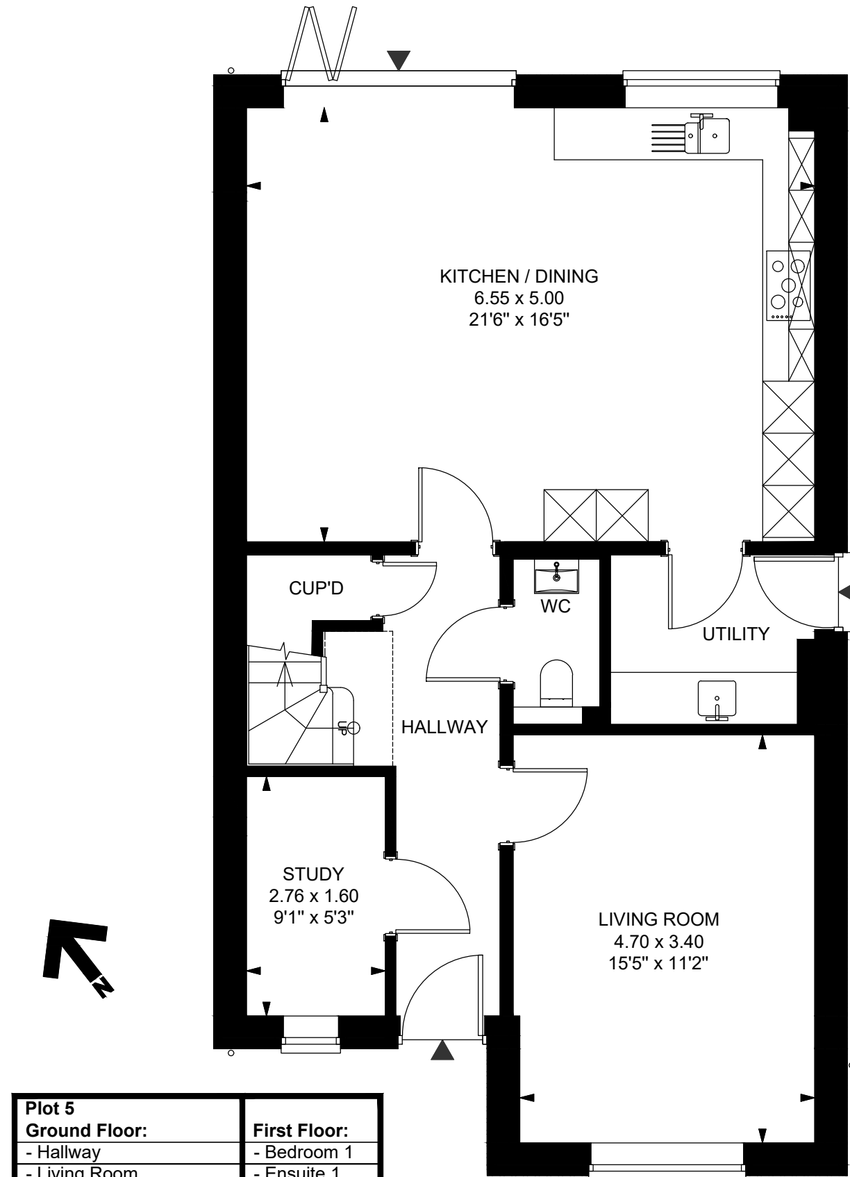
GROUND FLOOR (Plot 5) FOR MARKETING PURPOSES ONLY
