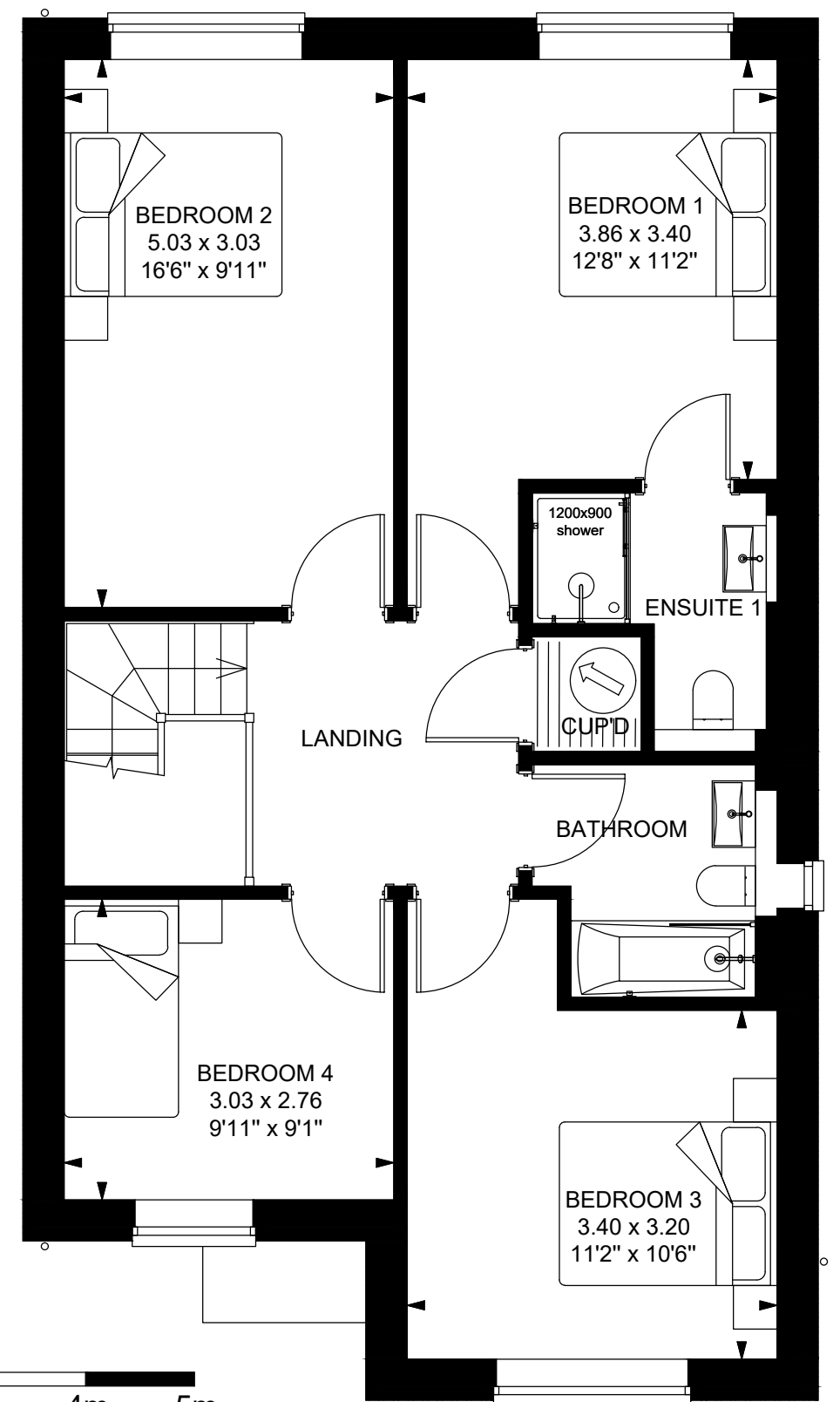
FIRST FLOOR (Plot 5) FOR MARKETING PURPOSES ONLY
